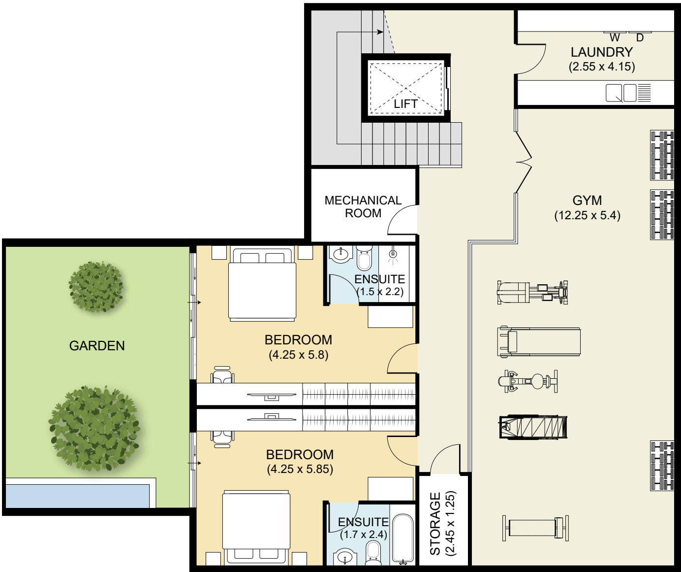
LOWER LEVEL
