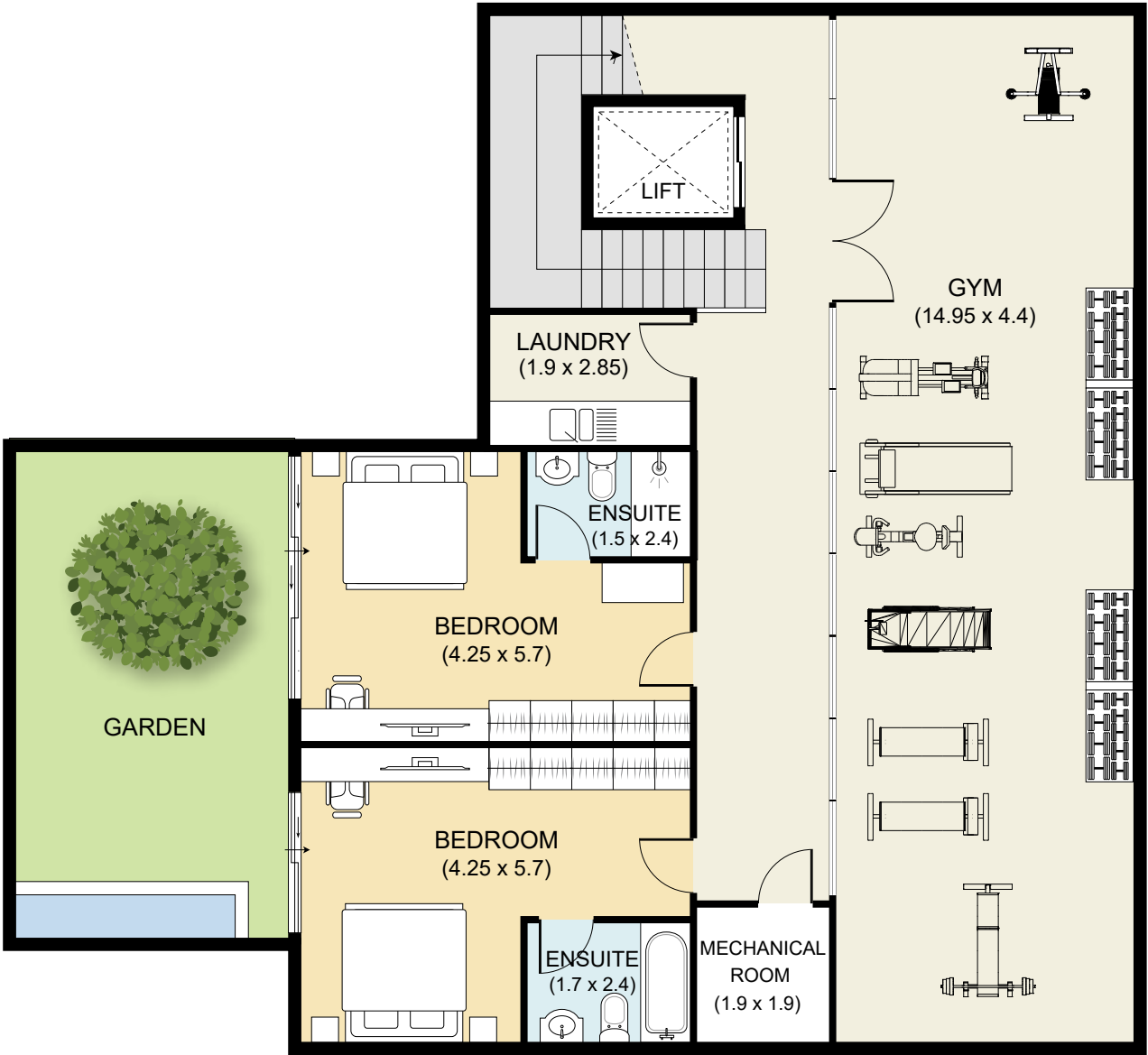
LOWER LEVEL
