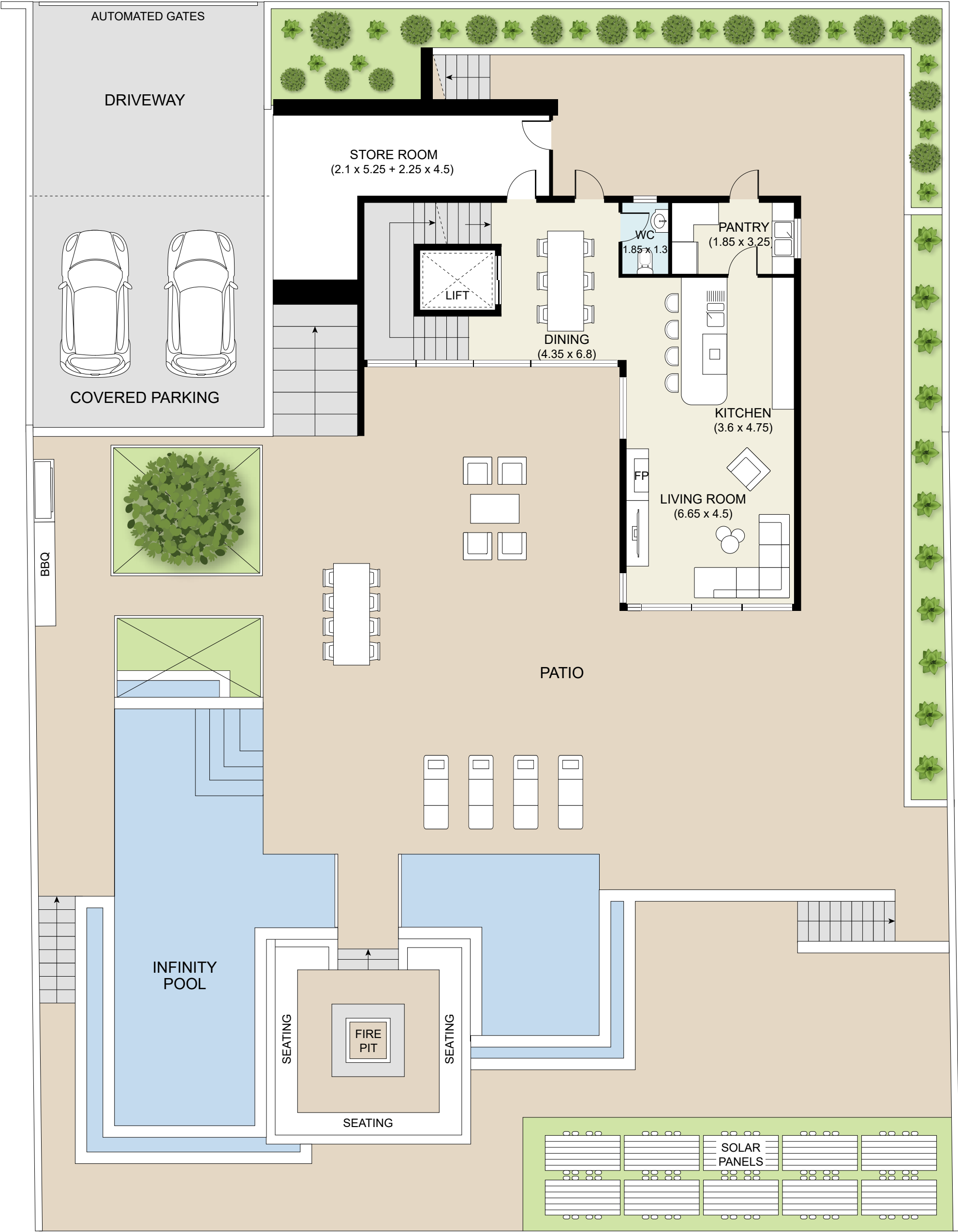
GROUND FLOOR
