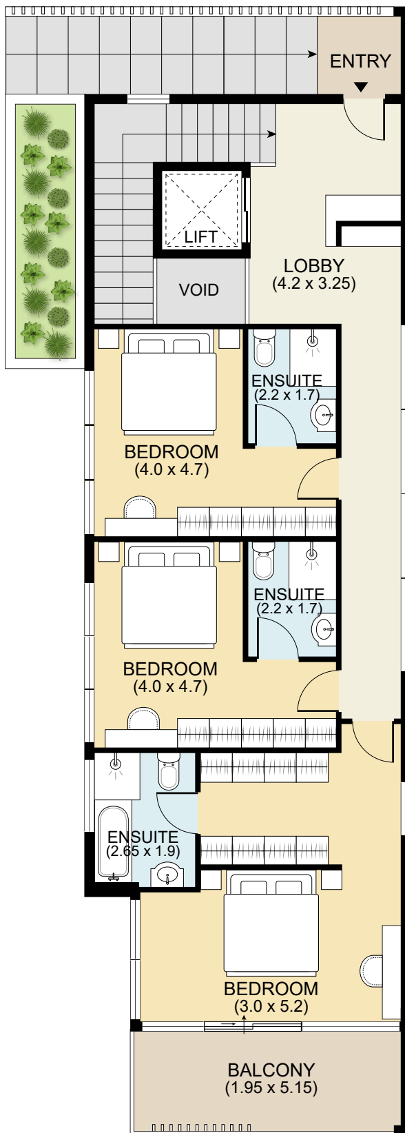
FIRST FLOOR
