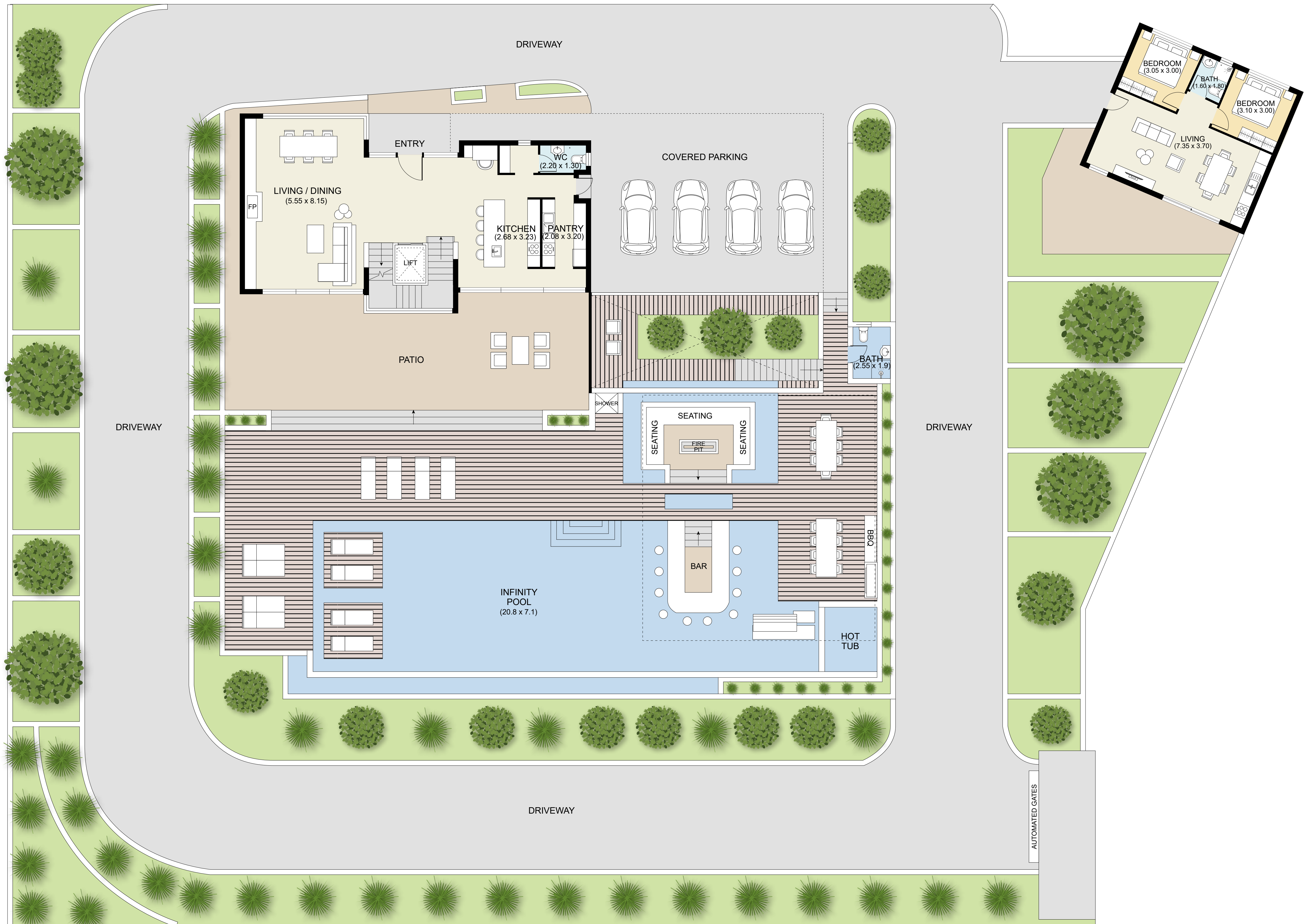
GROUND FLOOR
